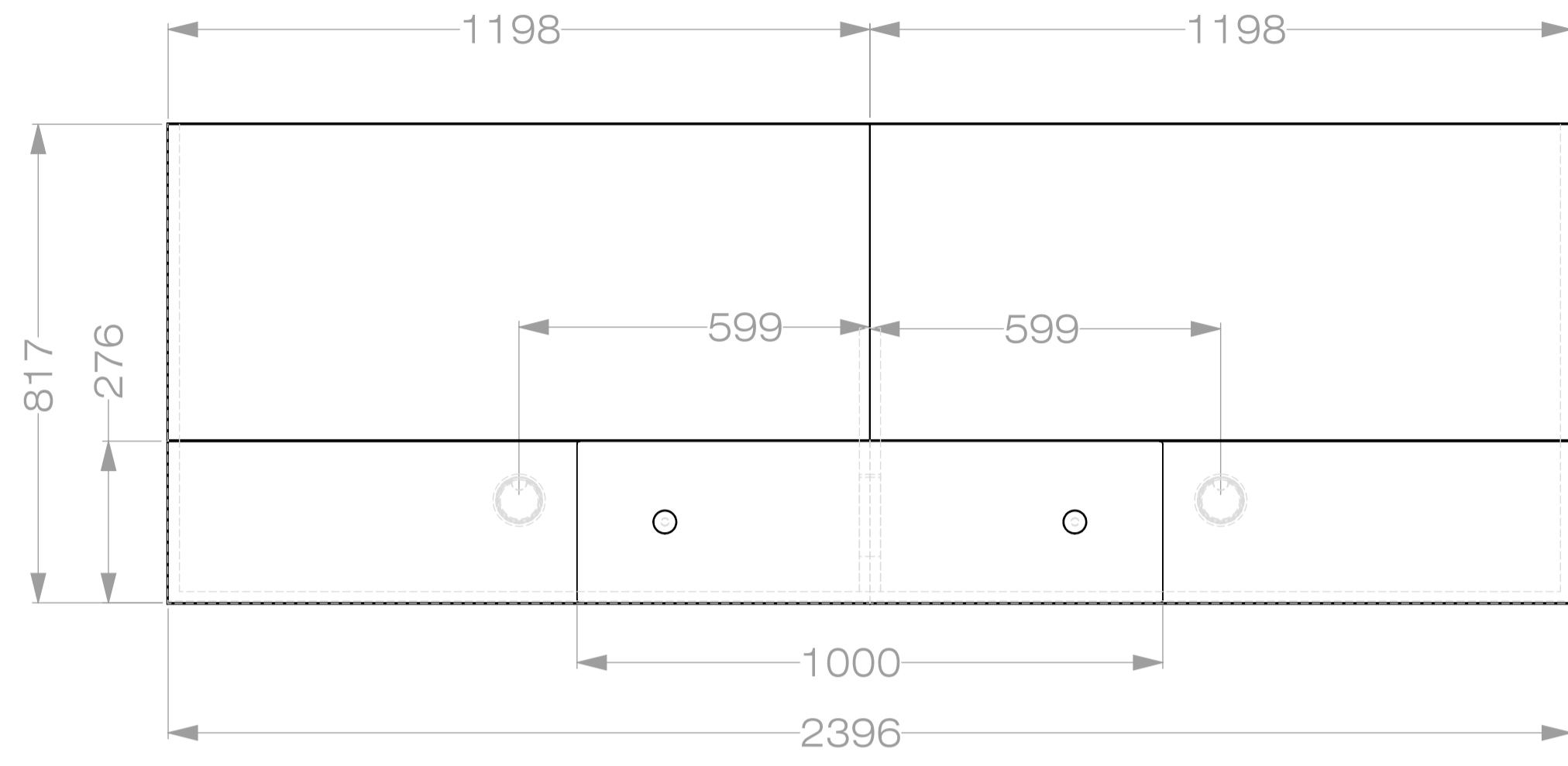
Drawing View2
