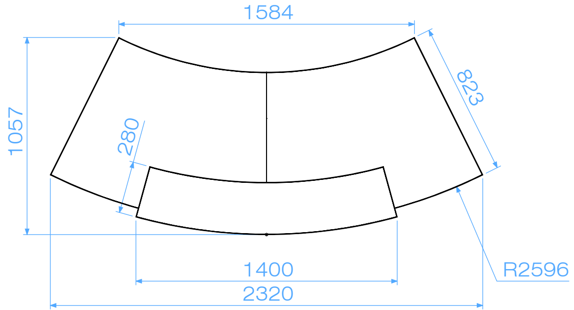
PLAN VIEW
