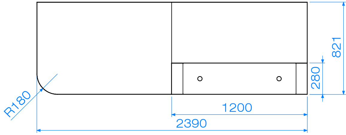
PLAN VIEW
