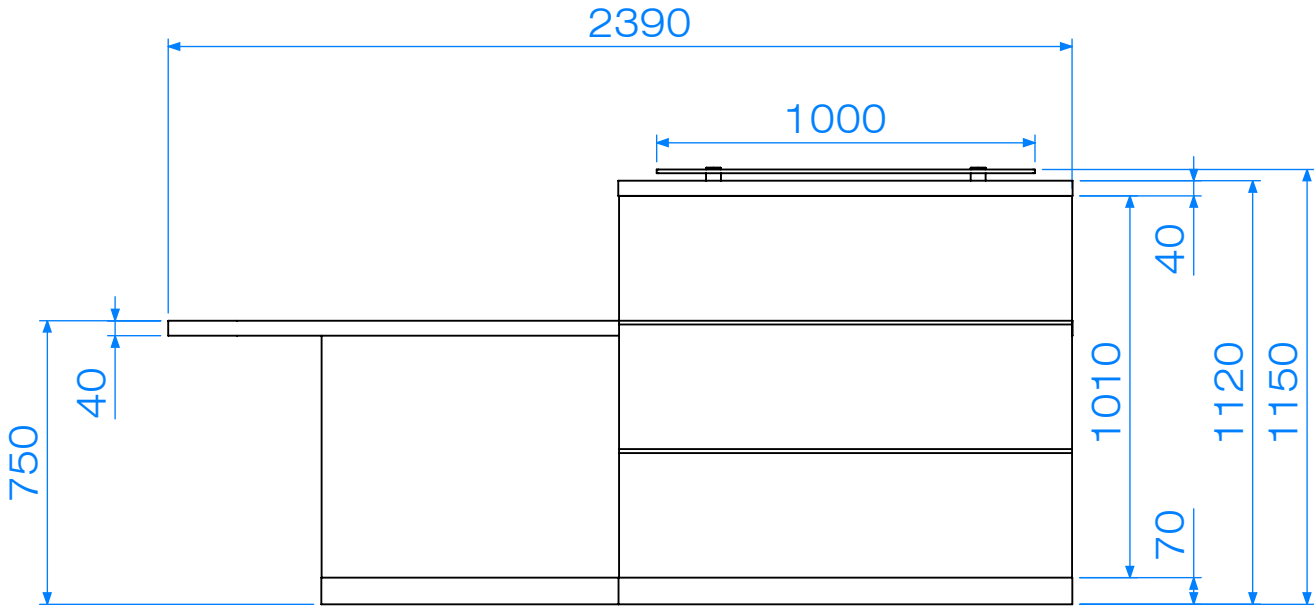
FRONT ELEVATION
