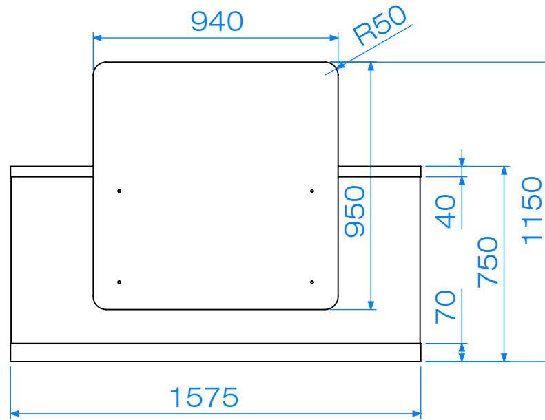
FRONT ELEVATION
