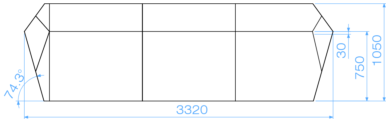
FRONT ELEVATION
