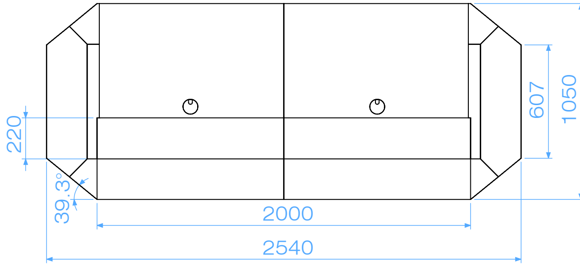
PLAN VIEW
