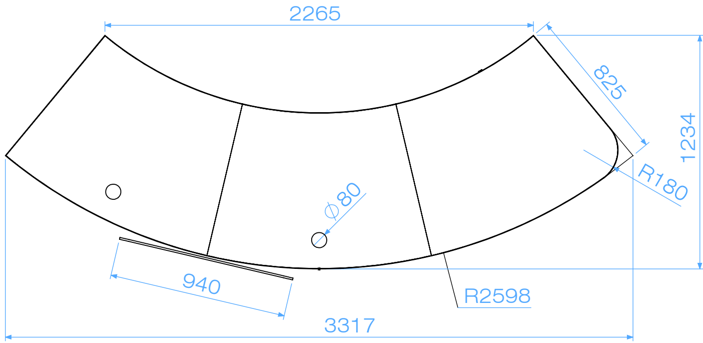
PLAN VIEW
