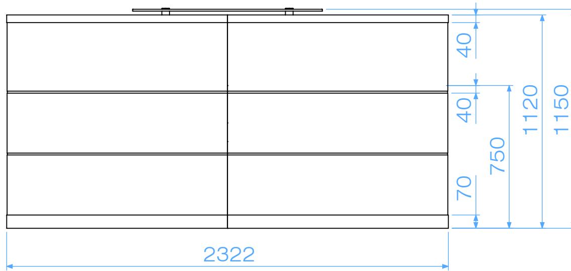
FRONT ELEVATION
