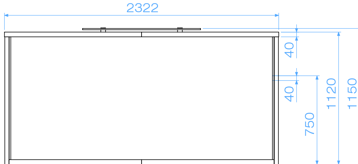
FRONT ELEVATION
