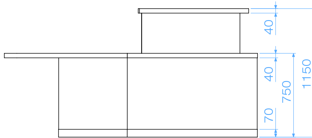
FRONT ELEVATION
