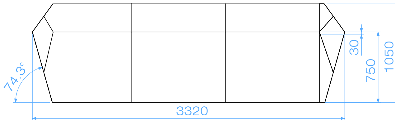
FRONT ELEVATION
