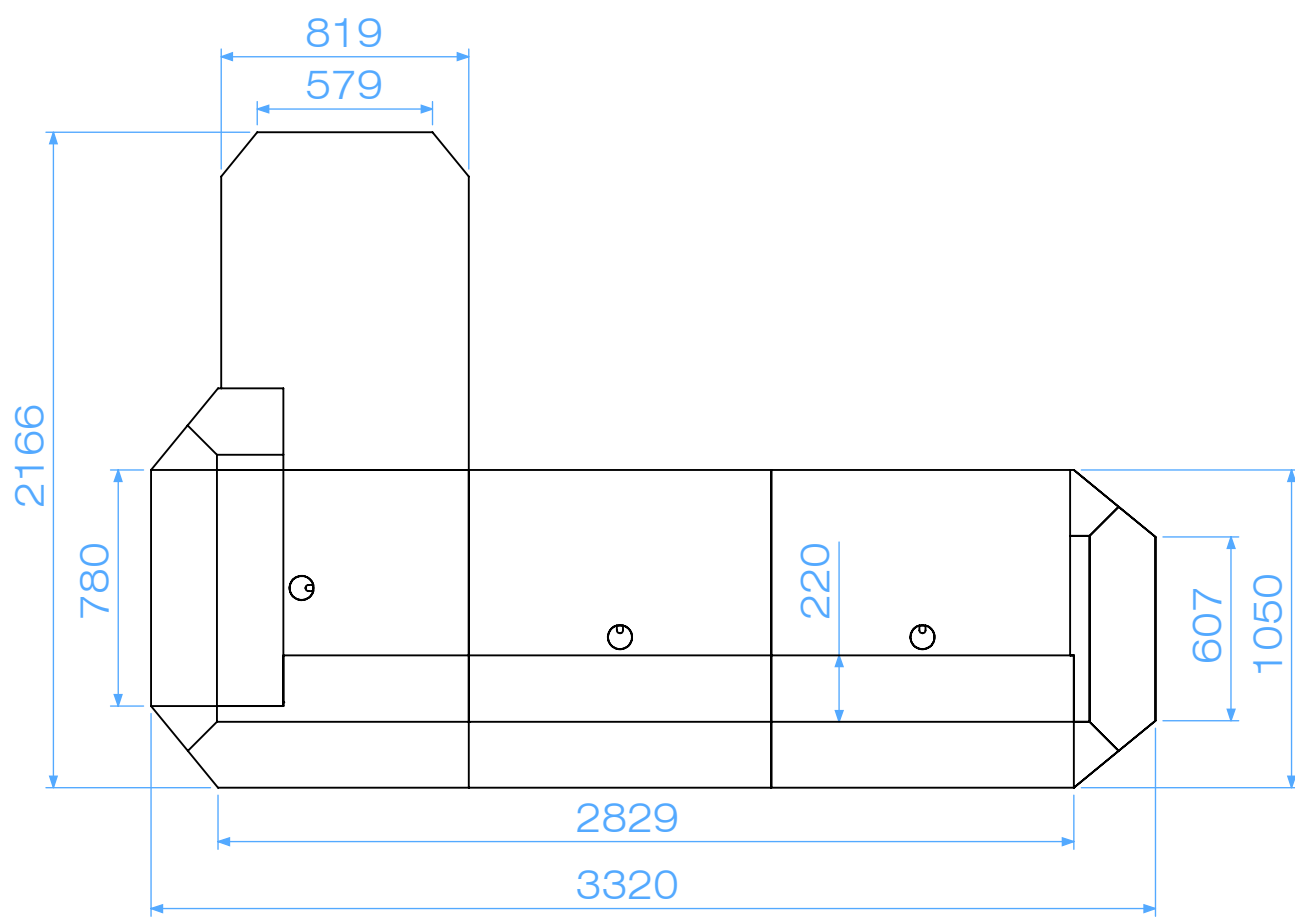
PLAN VIEW
