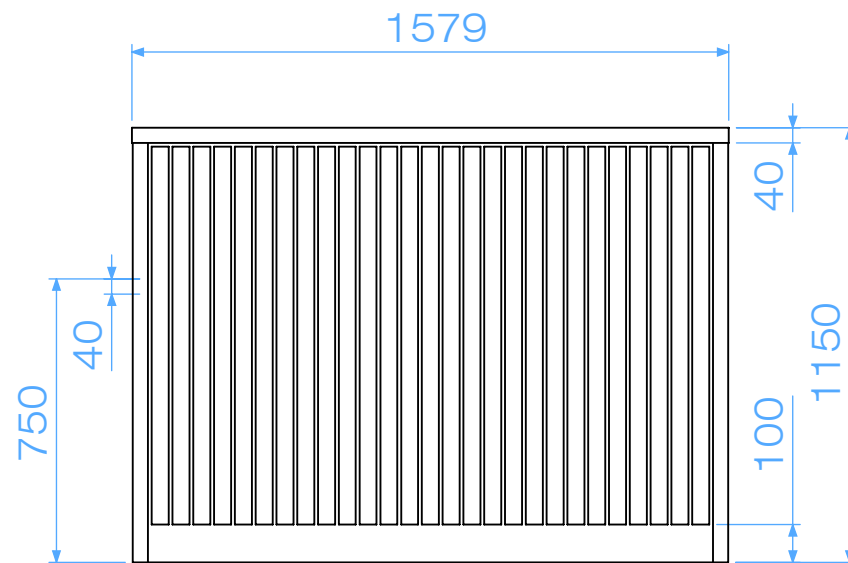
FRONT ELEVATION
