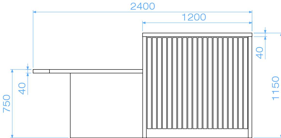
FRONT ELEVATION
